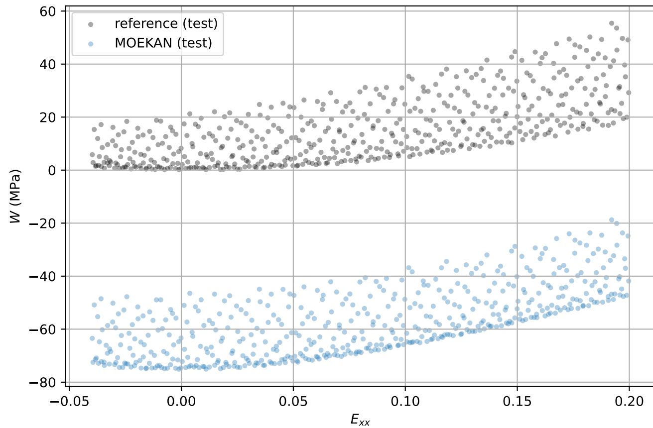
W versus E_{xx} (test)
