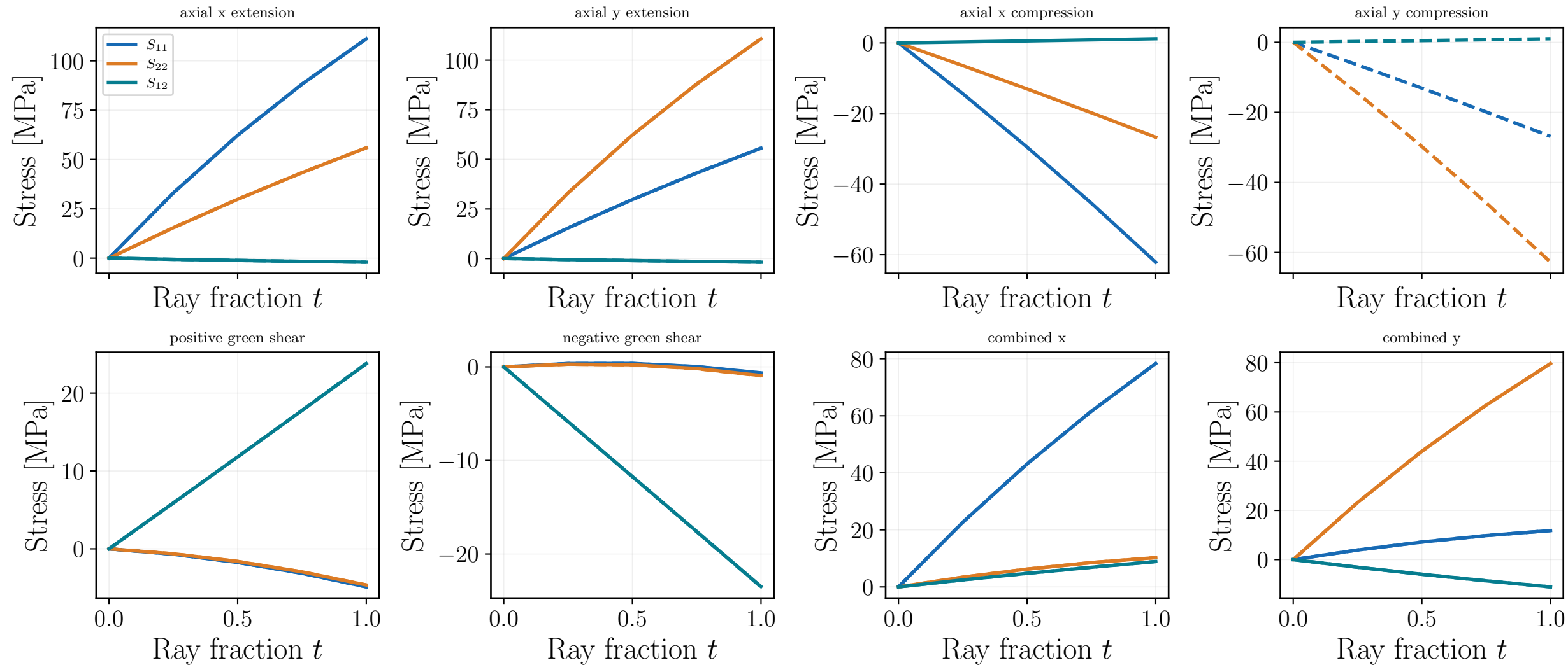
Material B FOM pilot: dashed coarse / solid fine; prescribed Green-strain rays
