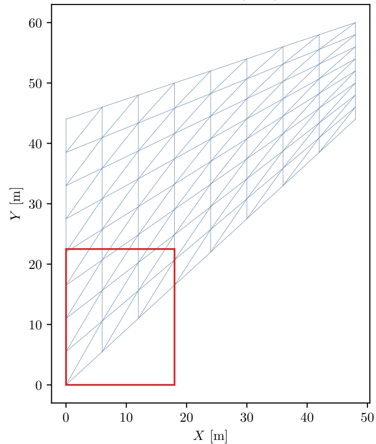
Cook's membrane: reference (undeformed) mesh 128 six-node quadratic triangles (Tri6), 384 Gauss points
