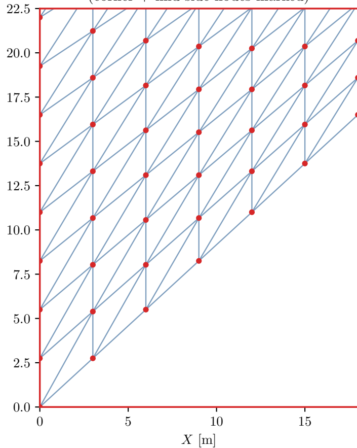
Zoom: individual Tri6 elements (corner + mid-side nodes marked)
