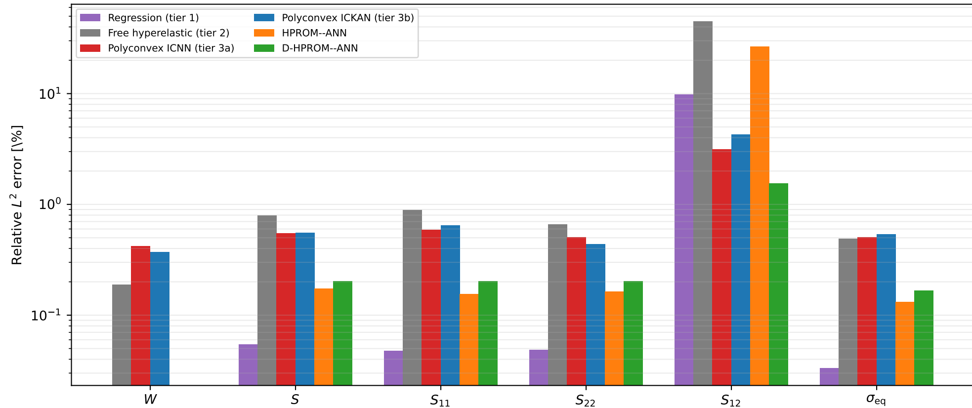
Stage--10 accuracy: all six model variants
