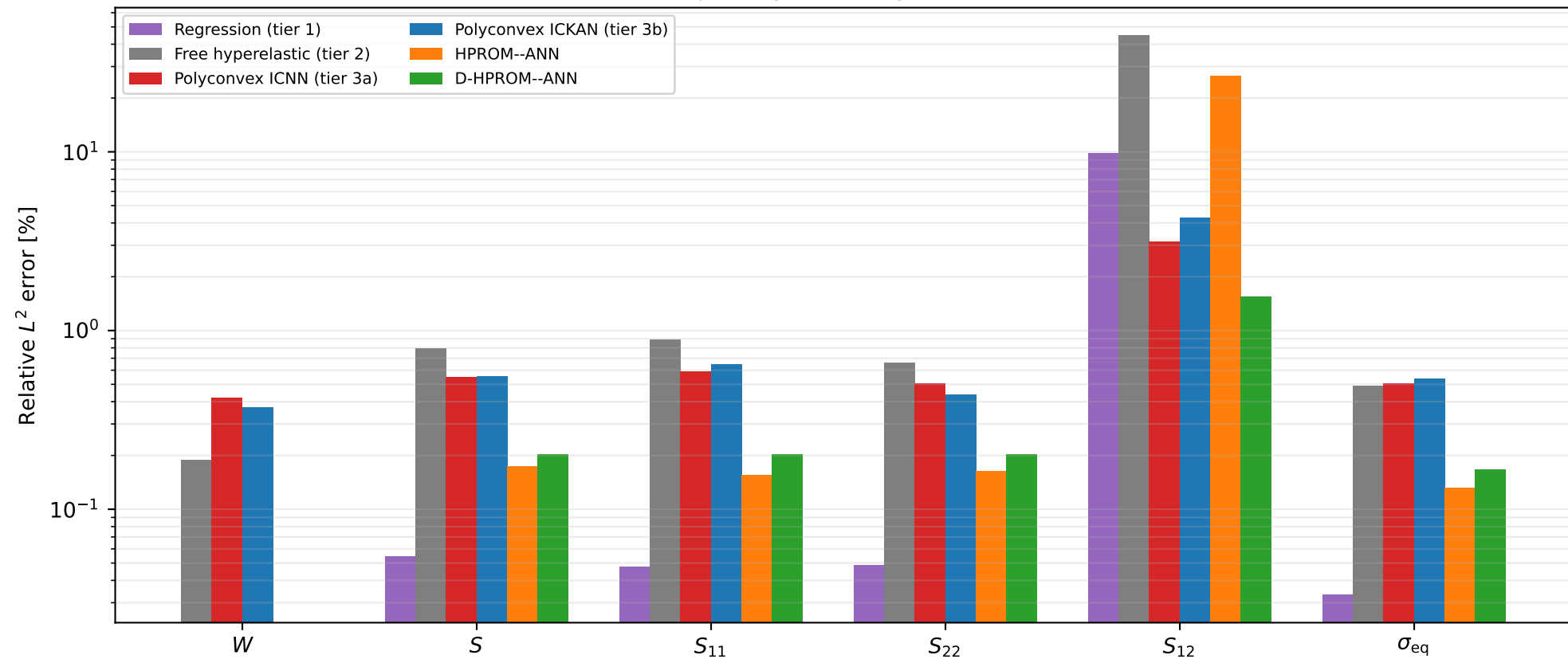
Held-out test-trajectory accuracy: all six model variants
