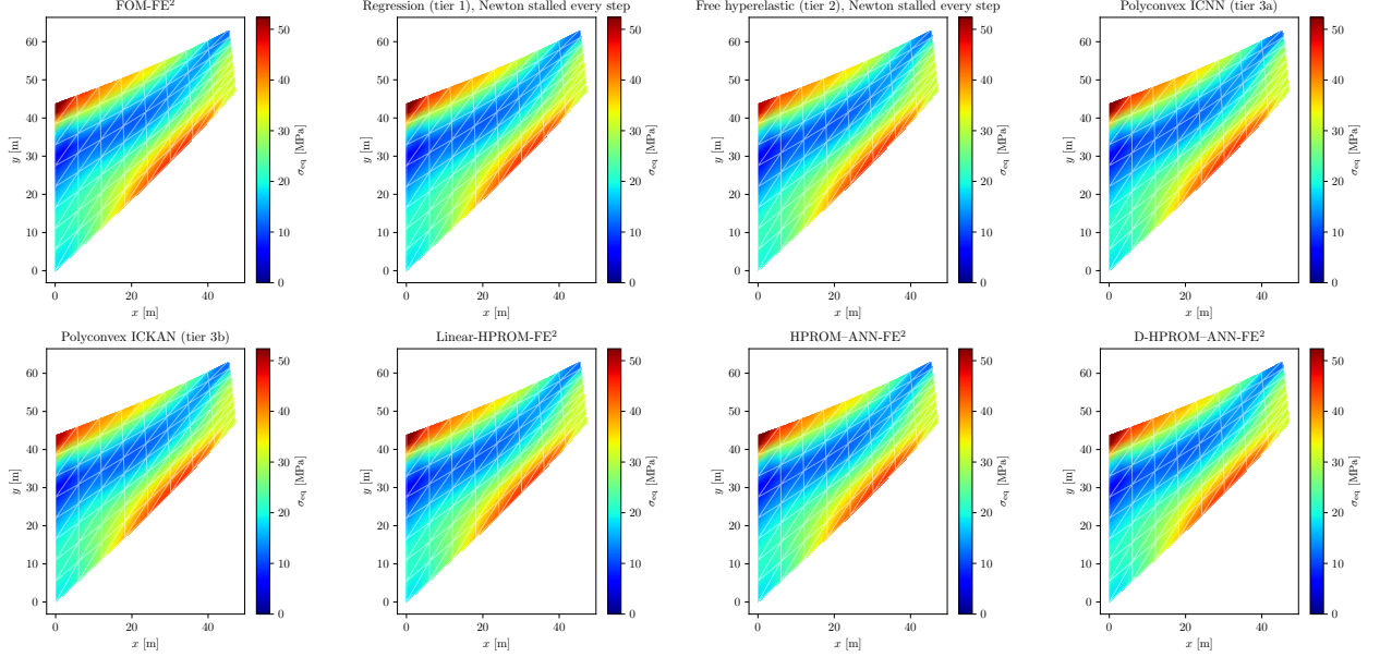
Cook’s membrane: equivalent (von Mises) stress field, every row of Table 7
