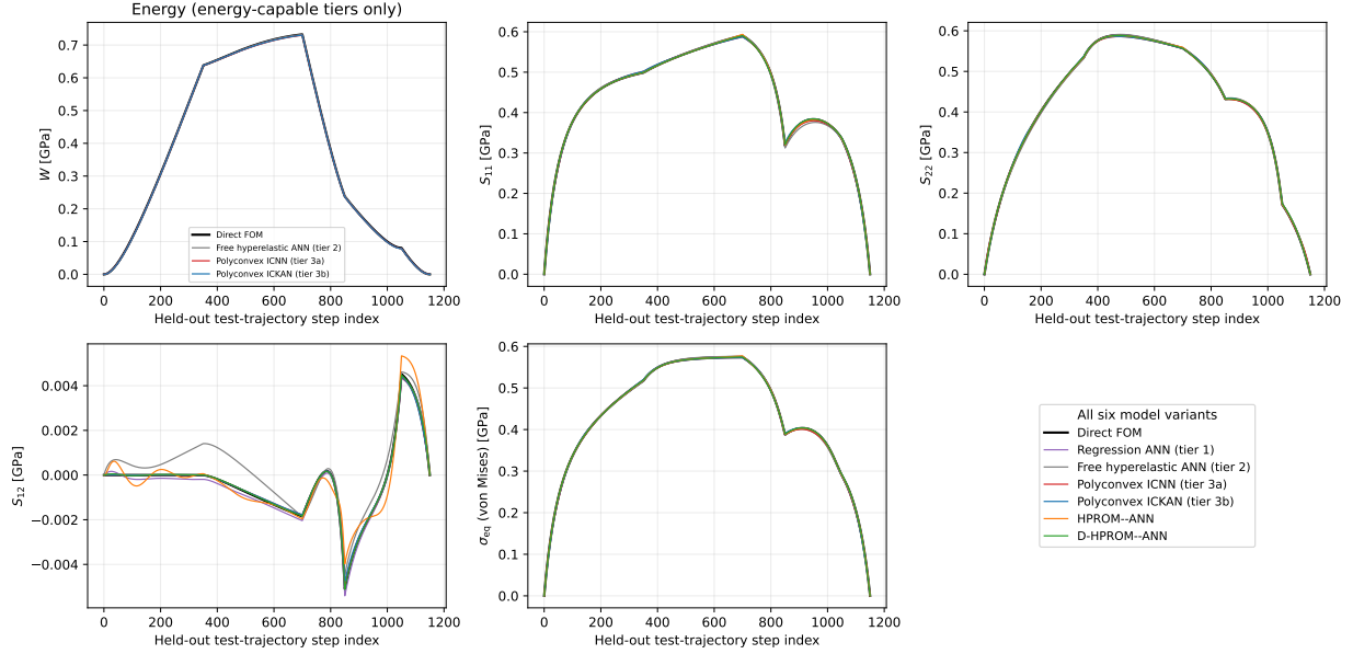
Figure 15: Test-trajectory comparison, direct FOM vs. all six model variants of Table 5 (the tier-1 pure-regression ANN, the tier-2 free hyperelastic ANN, the two certified polyconvex cores, and both HPRM-ANN operating modes): the three second Piola–Kirchhoff components S_{11} , S_{22} , S_{12} and the von Mises equivalent \sigma_{eq} , each shown for all six variants, plus energy W , shown only for the three energy-capable tiers (tier 2, tier 3a, tier 3b), since the tier-1 pure-regression model and both HPRM-ANN modes recover stress directly, without an underlying scalar potential, so no energy curve exists for them to plot (Section 6.5 for tier 1; Section 6.3’s discussion of the reaction-force procedure for the two HPRM-ANN modes). Every plotted variant is visually indistinguishable from the FOM and from each other on this test path (including the free model, whose lack of a polyconvexity certificate is not visible here), which is exactly why Sections 6.5 and 6.6 audit them directly (cyclic work, rank-one curvature) rather than relying on this figure.
