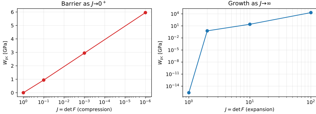
Figure 8: Total trained energy W_{\text{pc}} along the pure-dilatation path \mathbf{F} = \text{diag}(J, 1) : the logarithmic barrier acts as J \rightarrow 0^+ , and the energy grows steeply as J \rightarrow \infty . Along this path |\mathbf{F}| grows together with J , so the growth shown here for J \gg 1 is dominated by the sixth-power structural-stretch terms of Proposition 5, not by the volumetric term h(J) in isolation; see Figure 7 for that.
