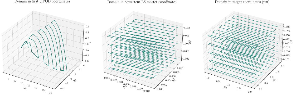
Figure 9: The training domain in three coordinate systems, all built from the same 109460 training-trajectory snapshots of this RVE. Left: the first three raw POD coordinates (q_{\text{tot},1}, q_{\text{tot},2}, q_{\text{tot},3}) , a curved, self-intersecting ribbon that is POD-optimal for reconstruction but not well suited to regression. Middle: the same snapshots in the structured, least-squares-fitted primary coordinates \mathbf{q} actually used as (35)’s input, recovering a near-affine, boustrophedon sweep. Right: the macro-strain domain itself, \boldsymbol{\varepsilon} = (E_{11}, E_{22}, \gamma_{12}) , for comparison. The middle and right panels are visually close by construction: that closeness is exactly the least-squares fit being verified, not assumed.
