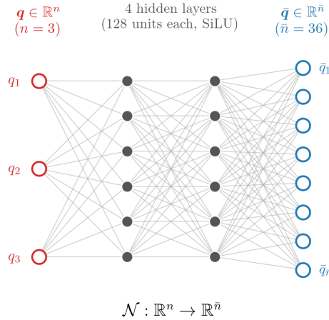
Figure 10: The decoder network \mathcal{N} : \mathbb{R}^n \rightarrow \mathbb{R}^{\bar{n}} of (35) for this RVE’s trained HPROM-ANN model ( n = 3 , \bar{n} = 36 ); only a representative subset of the 128 units per hidden layer is drawn.
