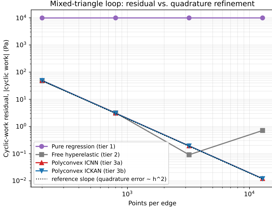
Figure 14: Residual magnitude on the mixed-triangle loop vs. quadrature points per edge, log-log, at the four refinement levels 200, 800, 3200, 12800. The three energy-based tiers fall on the slope expected of \mathcal{O}(h^2) trapezoidal quadrature error (dotted reference line) and are converging to the true value of exactly zero; the tier-1 residual does not move. The free-hyperelastic tier’s residual (tier 2, evaluated in float32) levels off around 10^{-1} – 1 Pa at the finest level rather than continuing to shrink, consistent with floating-point precision rather than remaining quadrature error; the two float64 tiers (3a/3b) keep converging cleanly throughout.
