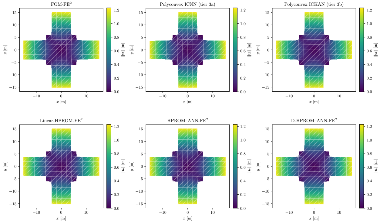
Cruciform specimen: real deformed states, six surviving models
