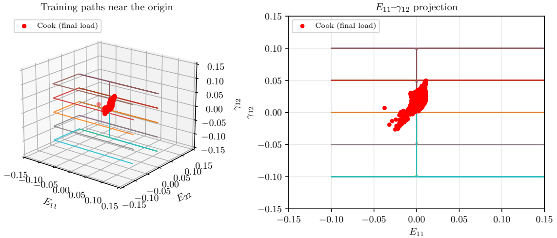
Figure 21: Training trajectories (colored, one per trajectory) against Cook’s own macro-strain states at full load (red), in the macro-strain coordinates (E_{11}, E_{22}, \gamma_{12}) near the origin. Left: a 3D view. Right: the E_{11} – \gamma_{12} projection, where each trajectory’s own fixed shear level appears as a horizontal line Cook’s cluster cuts across.
