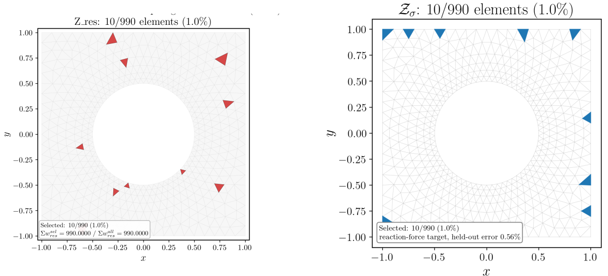
Figure 11: MAW-ECM hyperreduced integration supports for this RVE's canonical manifold-adaptive-weight configuration. Left: the |\mathcal{Z}| = 10 Gauss points retained for the projected equilibrium residual. Right: the |\mathcal{Z}_\sigma| = 10 Gauss points retained for the homogenized-stress output functional. The two supports are constructed independently and, as visible here, are not required to select the same elements.
