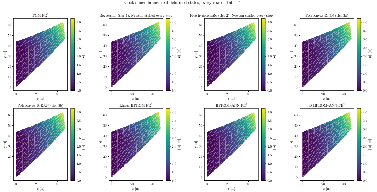
Figure 18: Cook’s membrane, real deformed configurations at full load, colored by displacement magnitude, every row of Table 7 in this paper’s canonical model order (FOM-FE 2 first). Every row, including the two uncertified tiers – pushed through the full ramp despite never converging per-step, not stopped at their own first stalled step – is visually indistinguishable from the true FOM.
