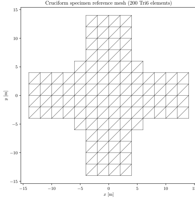
Figure 22: The cruciform specimen’s reference mesh (200 Tri6 elements), chosen by a mesh-convergence study with the cheap ICNN core as the macroscopic law: the sharp internal corners are a genuine, non-mesh-convergent geometric stress concentration, so this resolution is a tractability choice, not a converged one, and every row below is compared on the identical mesh rather than against its own converged limit.
