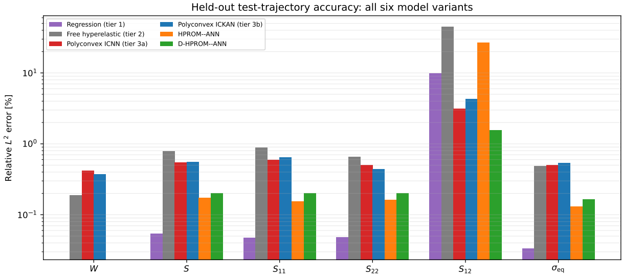
Figure 16: Test-trajectory relative L^2 error, all six reported quantities of Table 5, for all six model variants: the tier-1 pure-regression ANN, the tier-2 free hyperelastic ANN, the two certified polyconvex cores, and both HPRM-ANN operating modes. The uncertified ANNs (tiers 1–2) are competitive with, and on several components better than, the certified models on every accuracy metric shown here: consistent with Sections 6.5 and 6.6’s point that accuracy alone cannot distinguish a certified model from an uncertified one; only the cyclic-work and rank-one curvature audits can.
