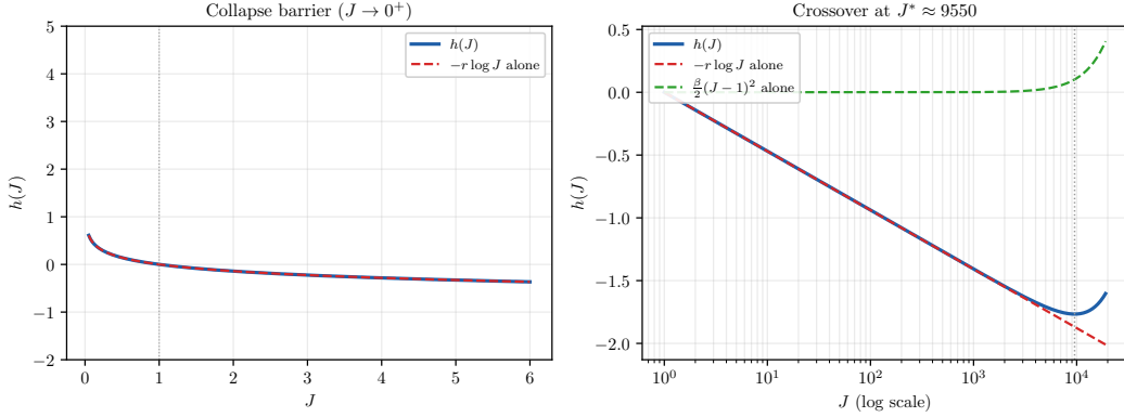
Figure 7: The volumetric barrier h(J) in isolation, with no feature or network terms and no coupling to a stretching path, for the trained coefficients r = 2.0390e - 01 , \beta = 2.2357e - 09 . Left: near J = 1 , h(J) and -r \log J alone are visually indistinguishable, and both diverge as J \rightarrow 0^+ . Right: on a log scale, -r \log J alone decreases without bound, and h(J) tracks it closely until the quadratic term alone finally overtakes it near J^* \approx 9550 , the point where h(J) starts to grow. This J^* is far beyond any dilation this RVE’s data ever reaches; the total trained energy nonetheless grows steeply for realistic stretches, driven by the sixth-power terms of Proposition 5 below rather than by h(J) itself (Figure 8).
