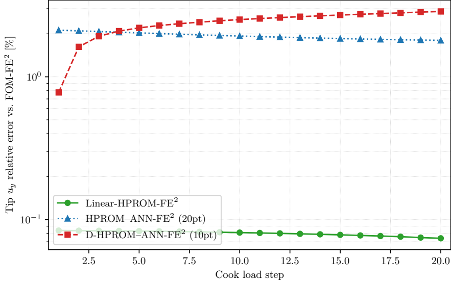
Figure 20: Tip u_y relative error against FOM-FE 2 , by load step, for the three rows sharing \phi_f : Linear-HPROM (no manifold ANN), HPROM-ANN (ANN prediction plus Newton correction), and D-HPROM-ANN (direct ANN prediction, no equilibrium correction).
