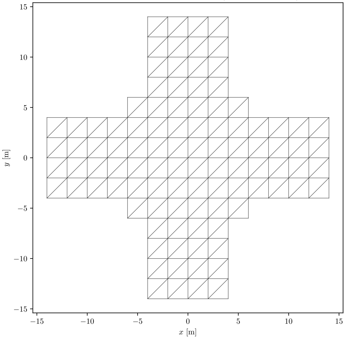
Cruciform specimen reference mesh (200 Tri6 elements)
