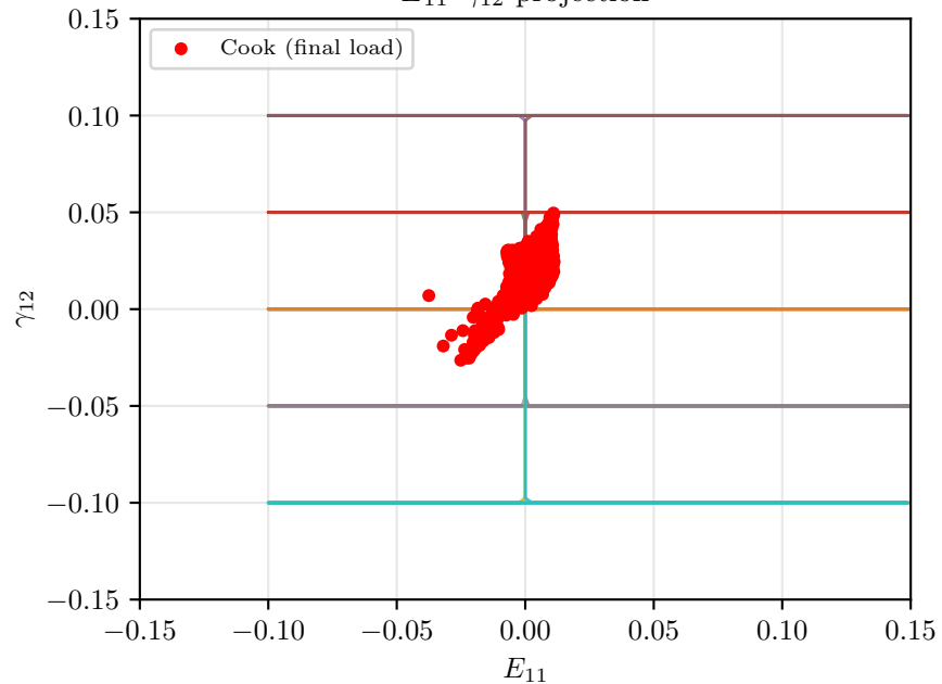
E_{11} - \gamma_{12} projection
