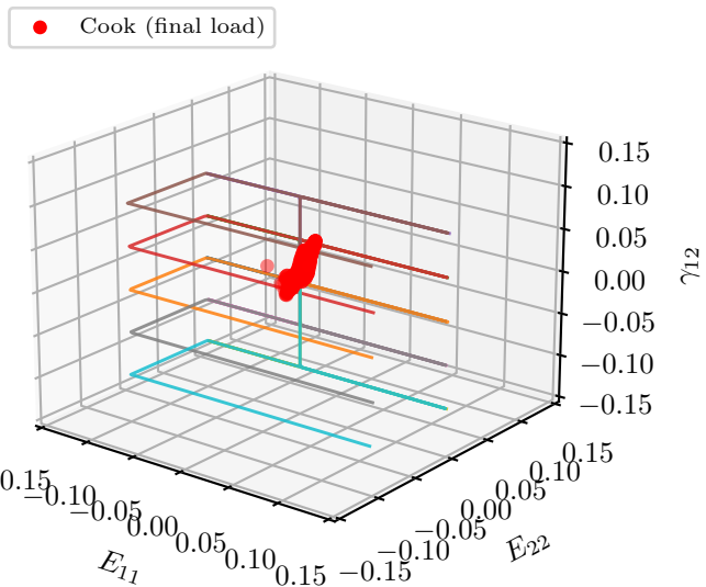
Training paths near the origin
