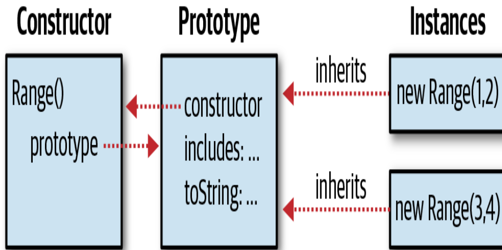
Figure 9-1. A constructor function, its prototype, and instances
