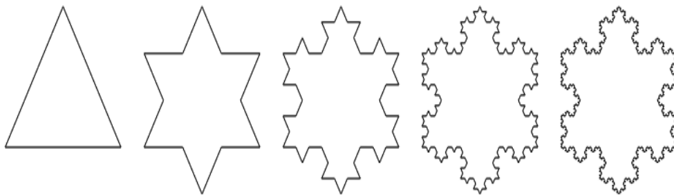
Figure 15-12. Koch snowflakes
