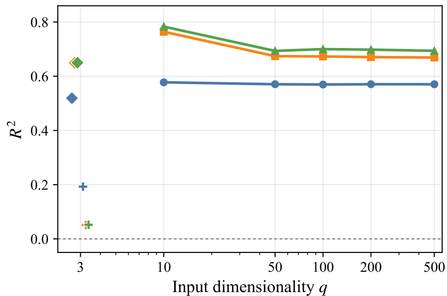
(c) Sparse PCA, Task f_D : St_{\text{act}} regression
