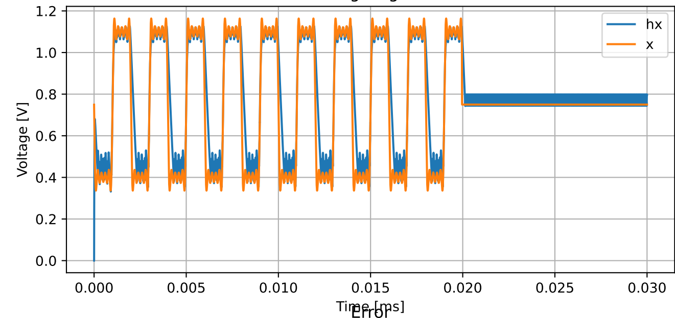
Voltage signals
