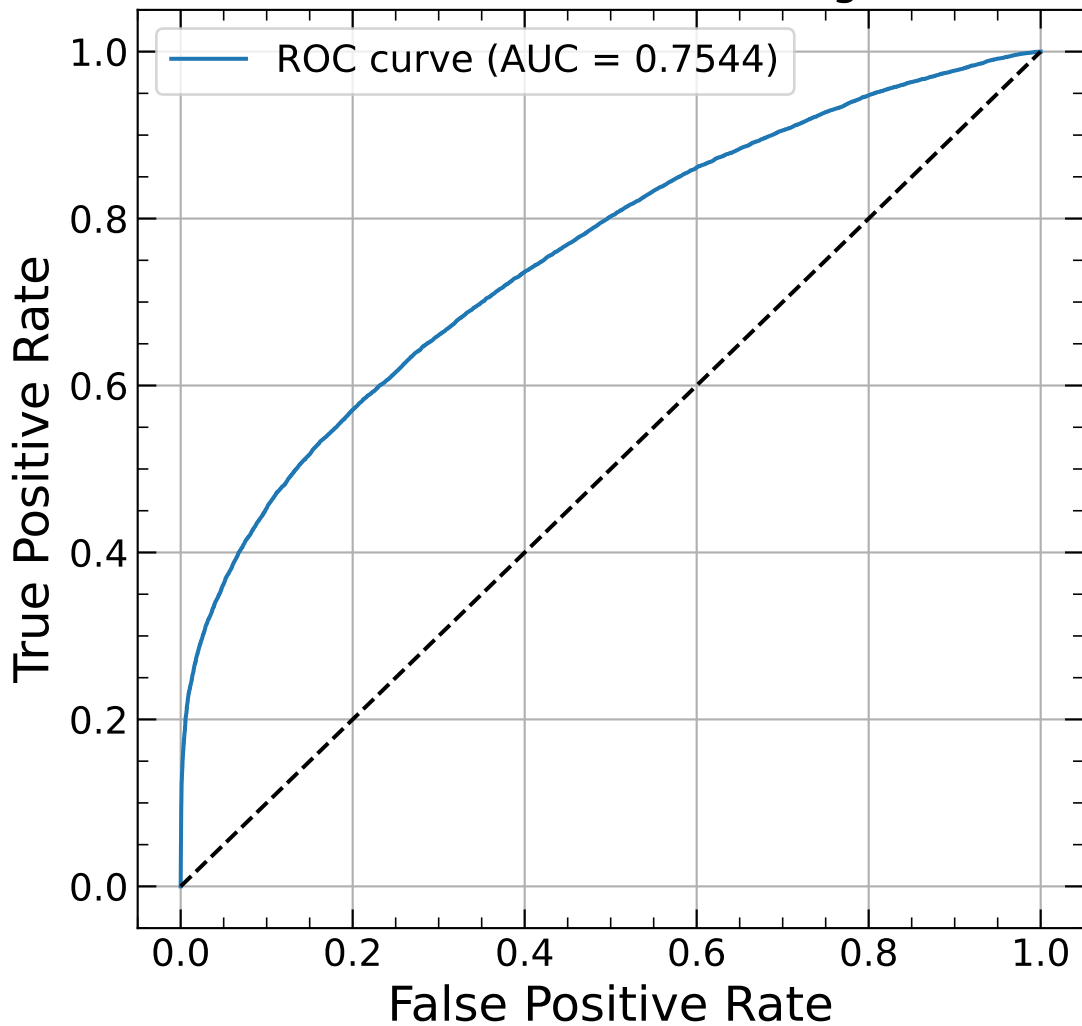
ROC Curve for MUON Background
