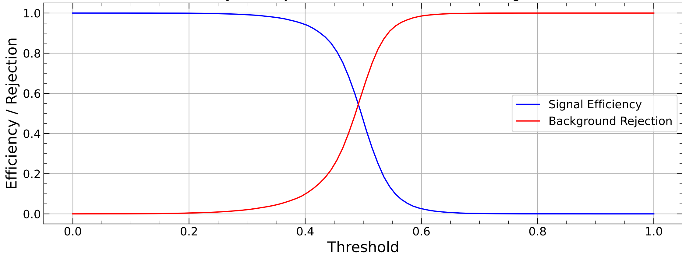
Efficiency and Rejection vs Threshold for KL0 Background
