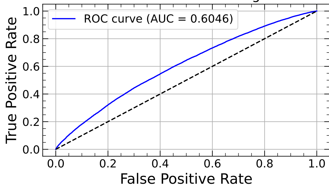
ROC Curve for MUON Background
