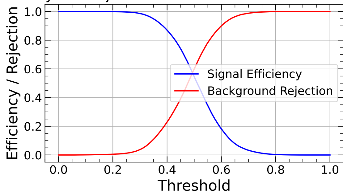
Efficiency and Rejection vs Threshold for MUON Background
