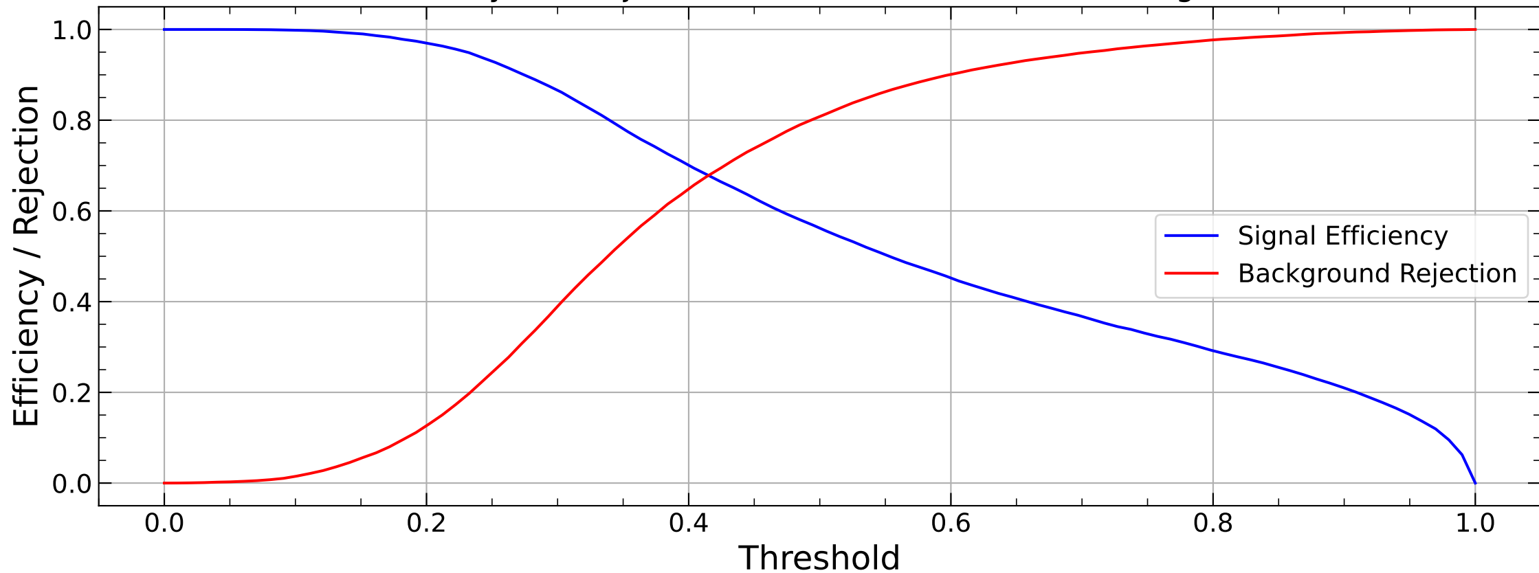
Efficiency and Rejection vs Threshold for MUON Background
