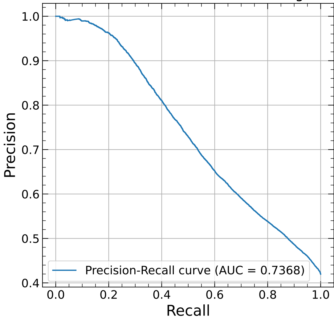
Precision-Recall Curve for MUON Background
