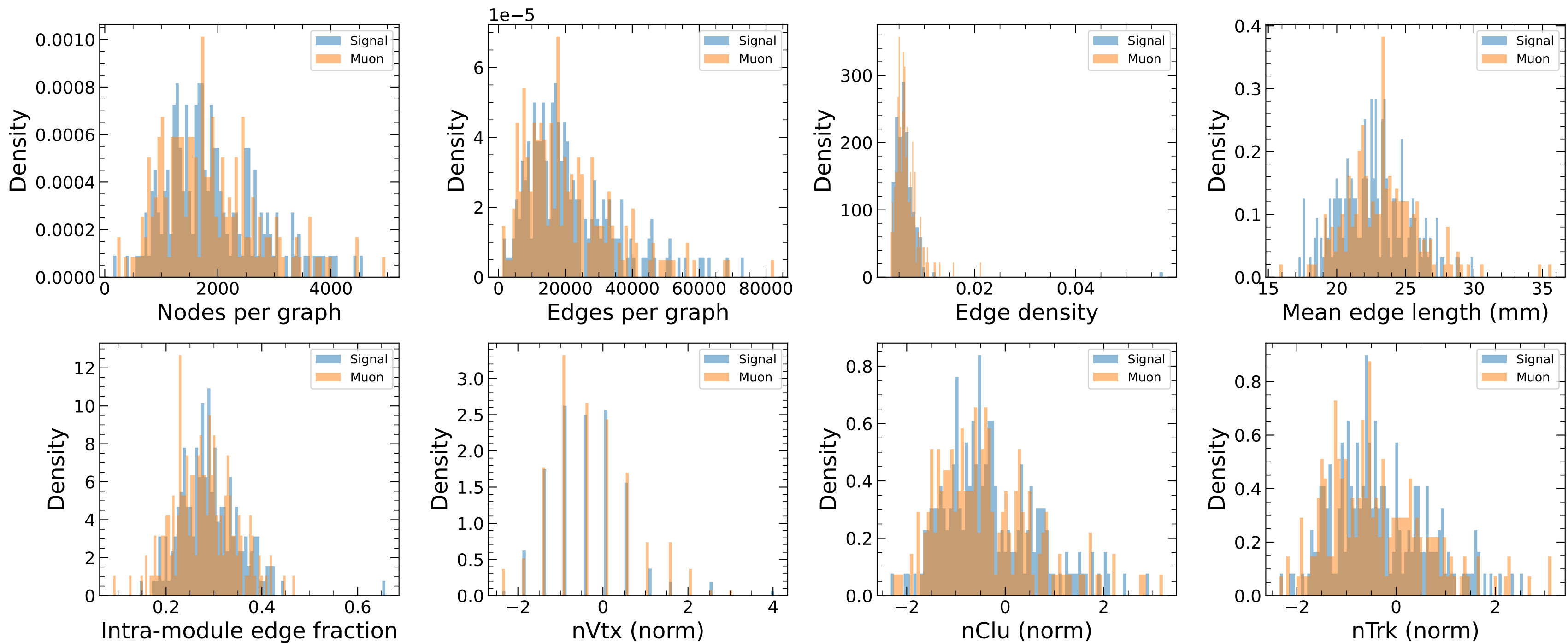
Graph-level stats — chunk 1, 200 evts/class
