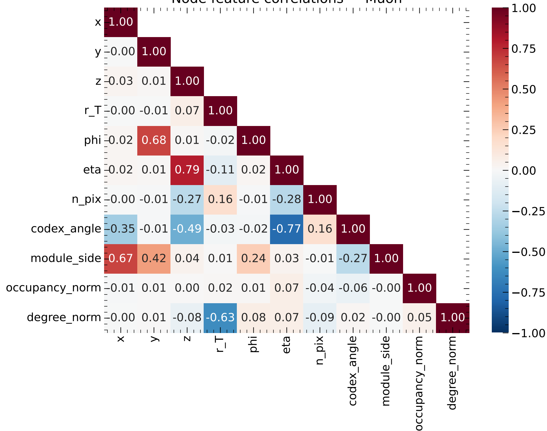
Node feature correlations — Muon
