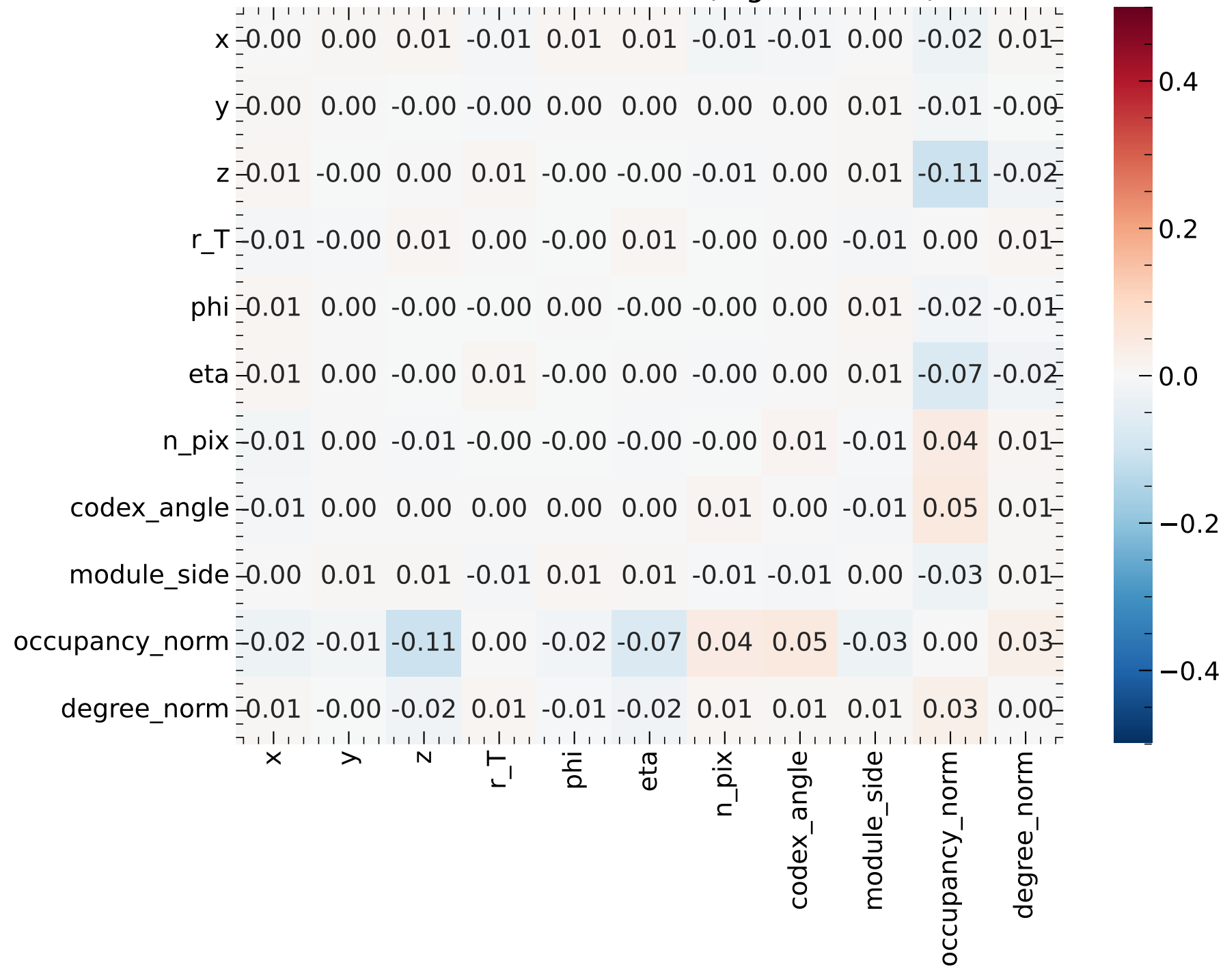
Correlation difference (Signal - Muon)
