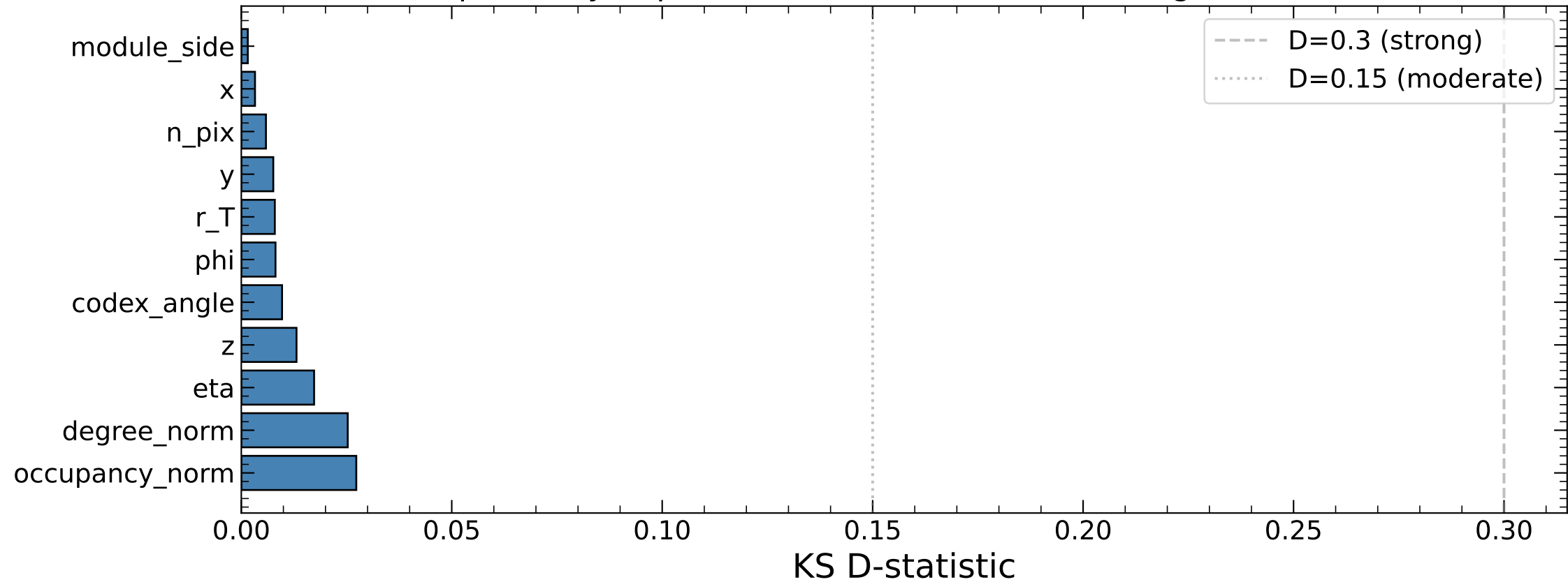
Separability of pooled node features (KS test: Signal vs Muon)
