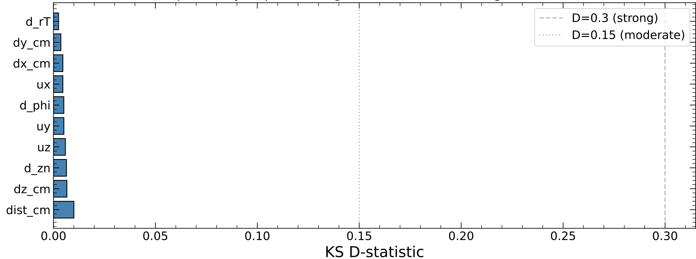
Separability of pooled edge features (KS test: Signal vs Muon)
