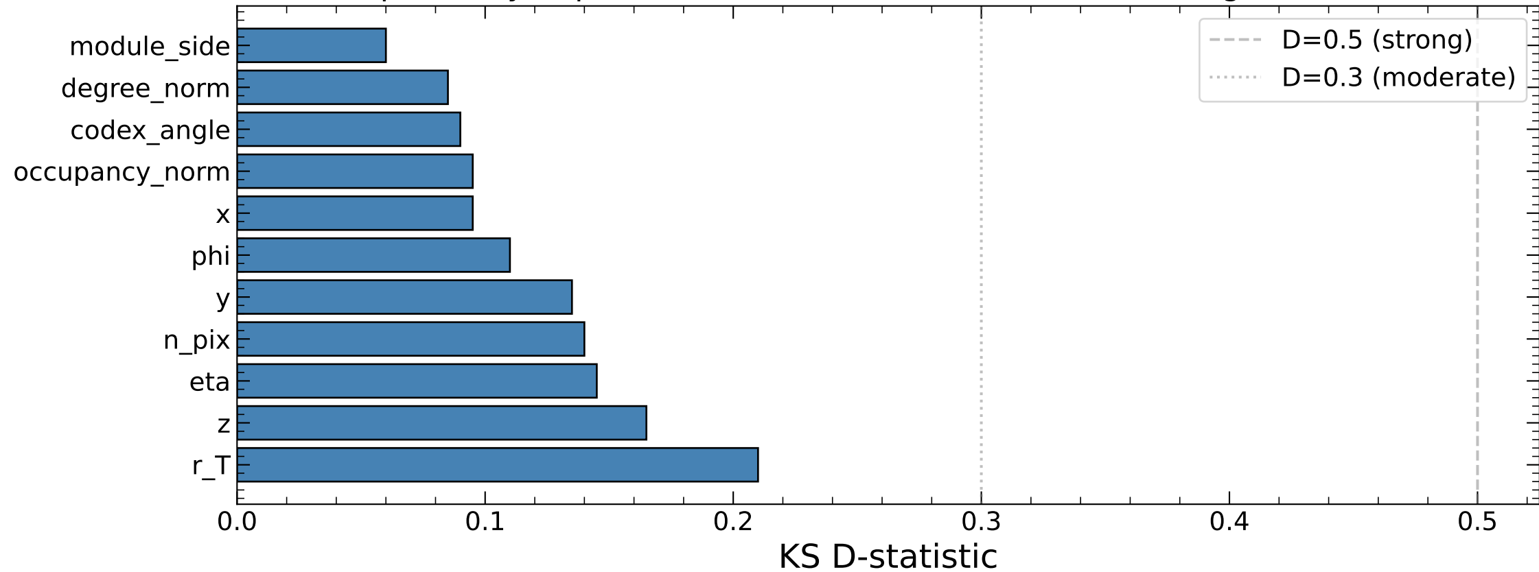
Separability of per-event mean node features (KS test: Signal vs Muon)
