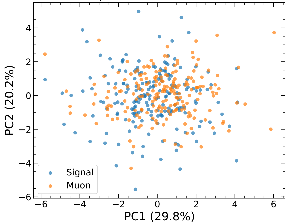
PCA on per-event mean node features
