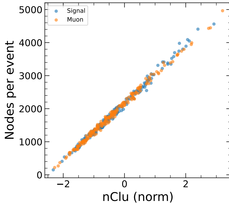
Global attributes vs event size
