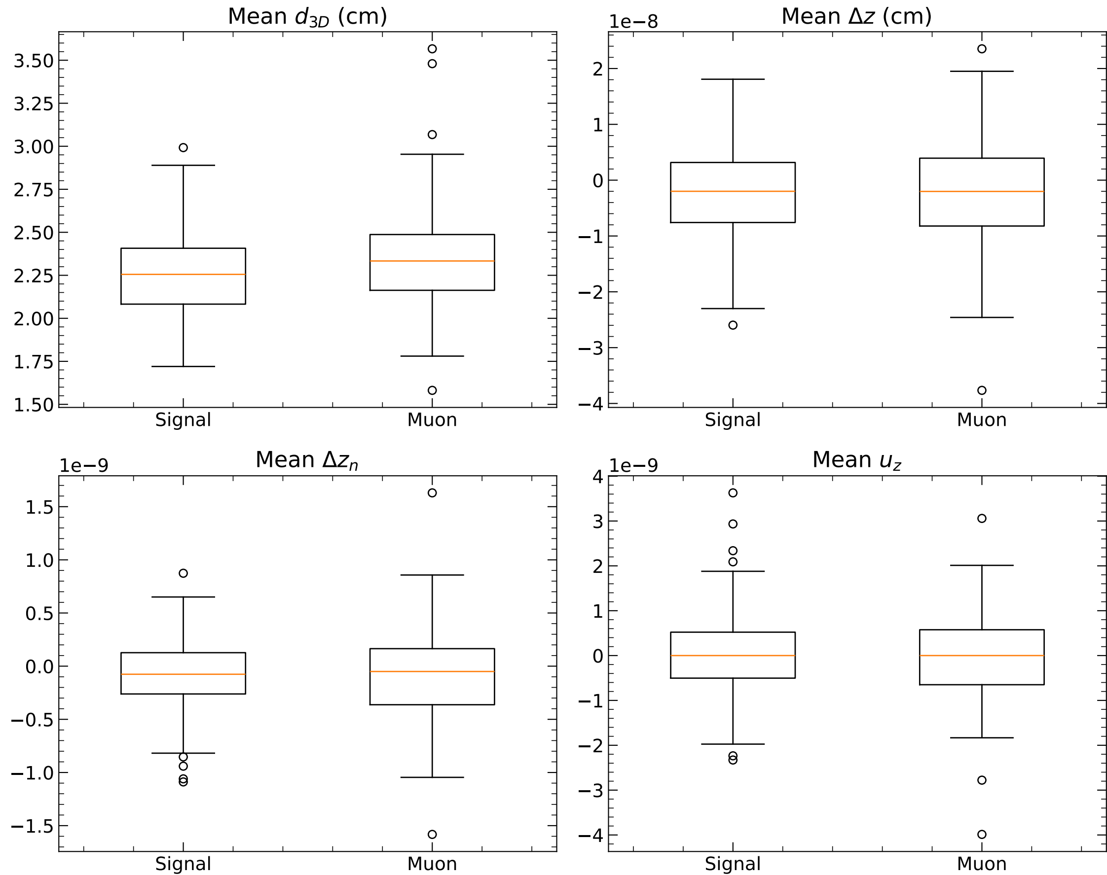
Top-4 most separating edge features (per-event mean)
