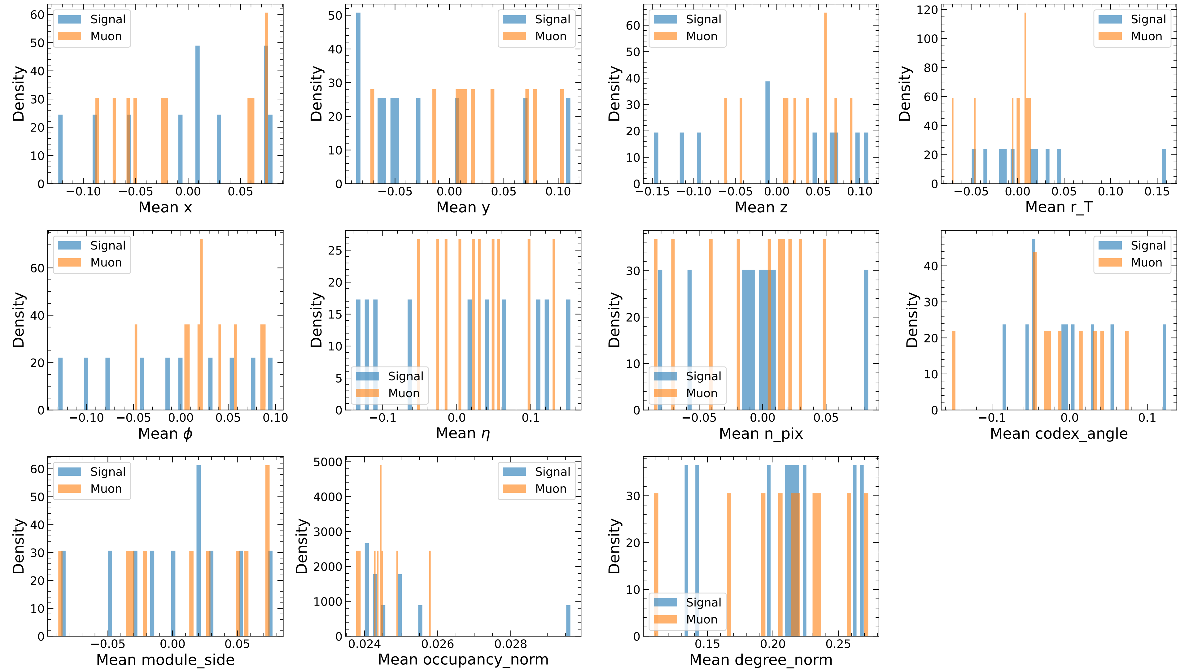
Per-event mean node features — Chunk 1
