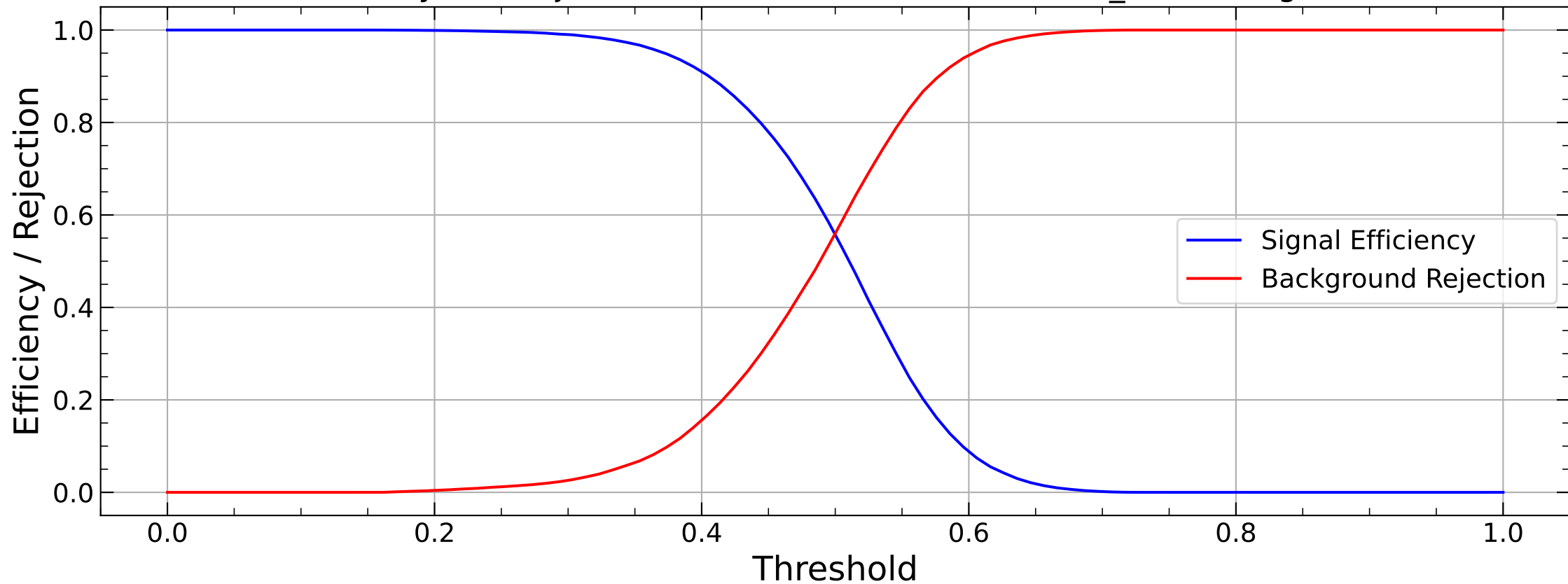
Efficiency and Rejection vs Threshold for SEPPARATE_BKG Background
