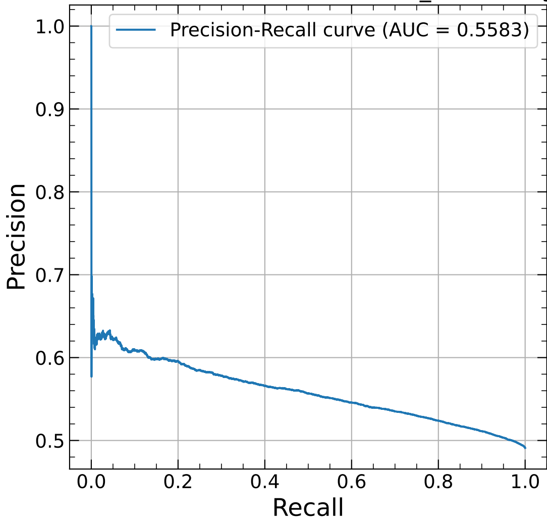
Precision-Recall Curve for SEPPARATE_BKG Backgro
