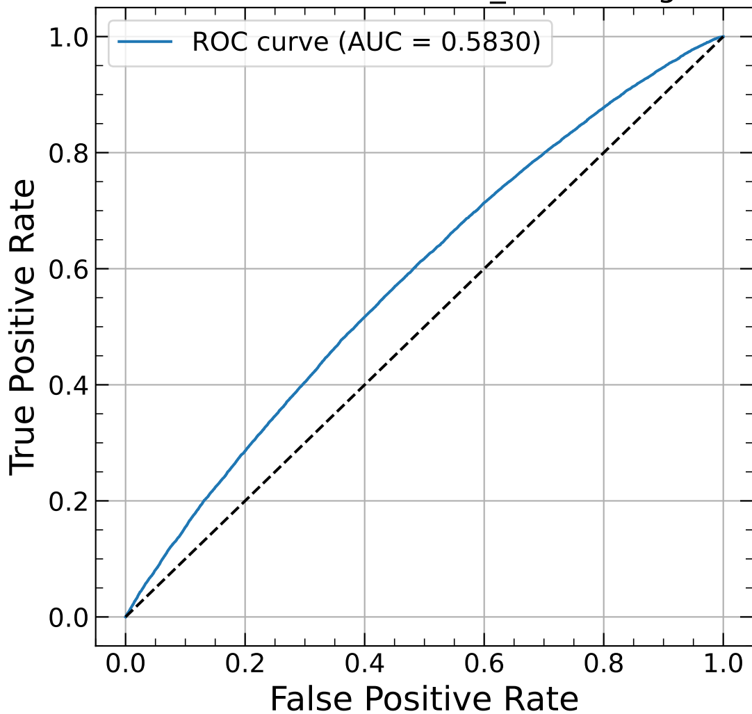
ROC Curve for SEPPARATE_BKG Background
