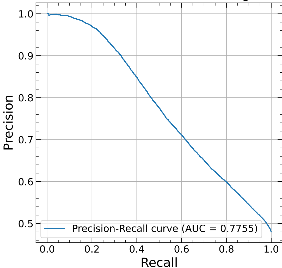
Precision-Recall Curve for KL0 Background
