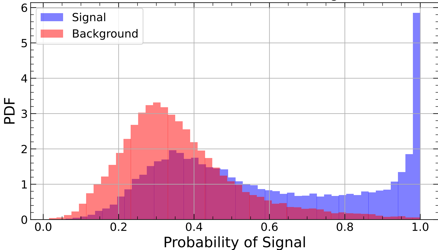
Predicted Probabilities for KL0 Background
