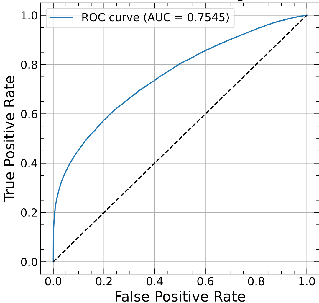
ROC Curve for KL0 Background
