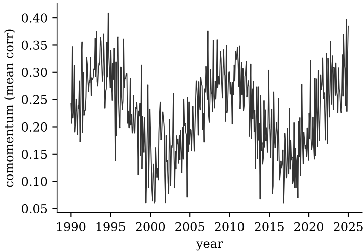
Comomentum (Stooq US)
