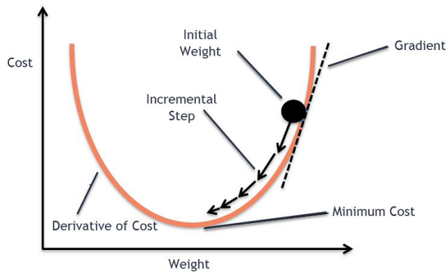
Figura 11. Gradient Descent
