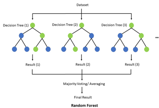
Figura 15. Random Forest
