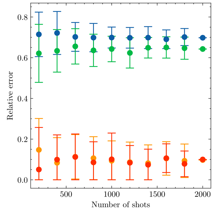
Non-local Pauli
