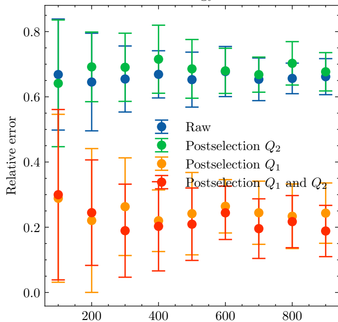
Energy
