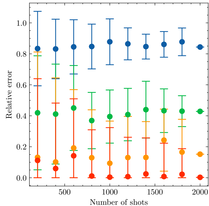
Non-local Pauli
