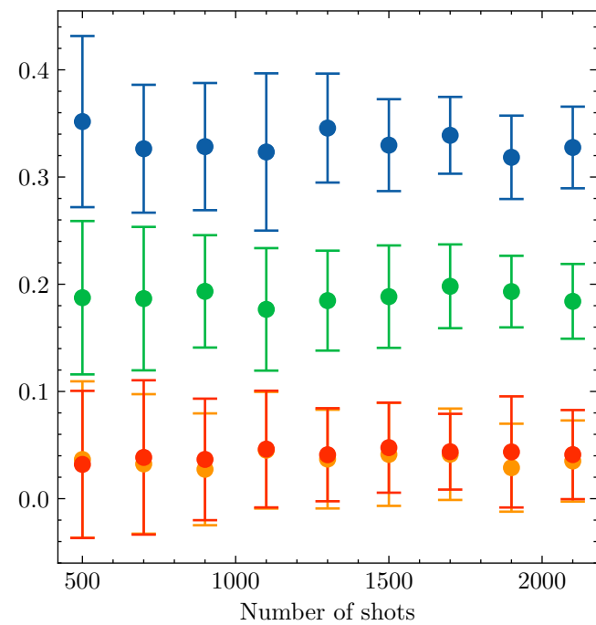
Non-local Pauli
