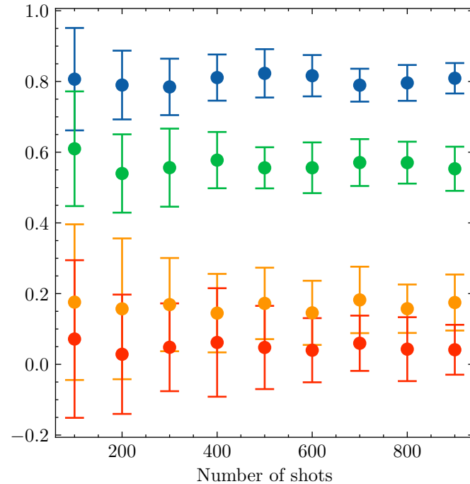
Non-local Pauli
