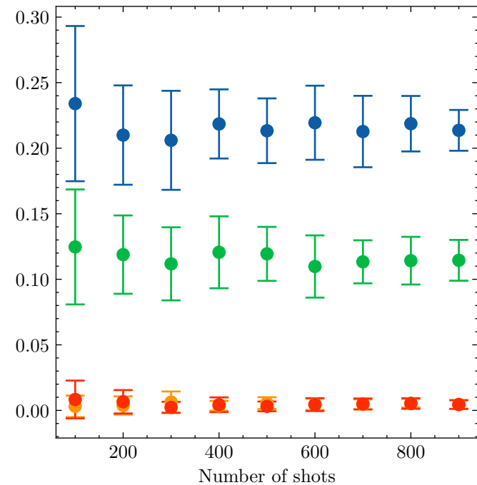
Non-local Pauli
