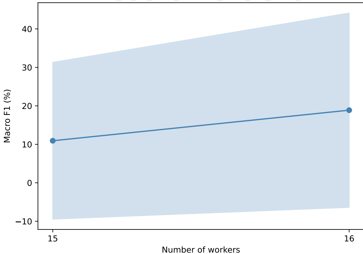
macro_f1_vs_num_workers_drop_0.0_mom_0.0
