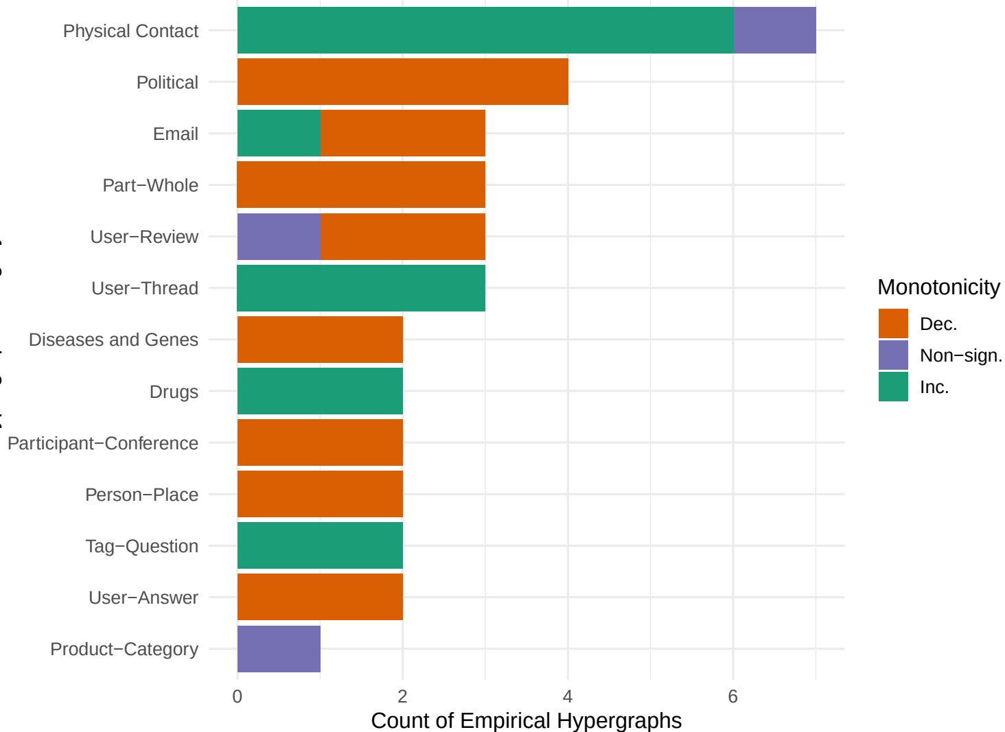
Monotonic Trend Direction by Hypergraph Category
