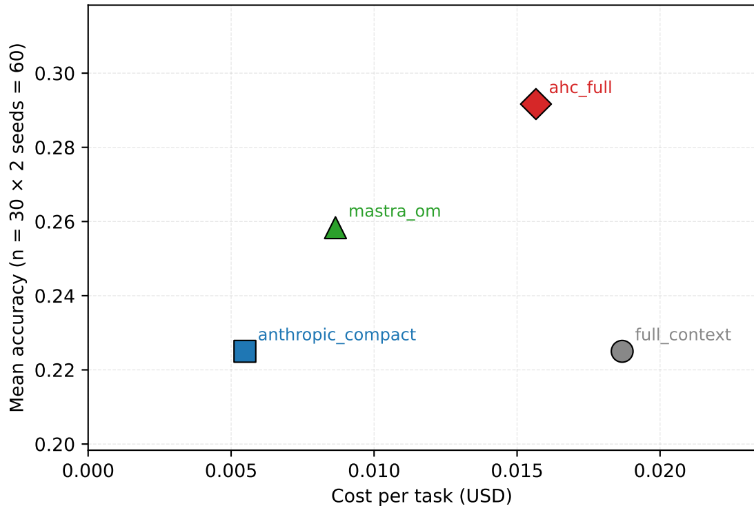
AssistantTraj — accuracy × cost (E1 main sweep)
