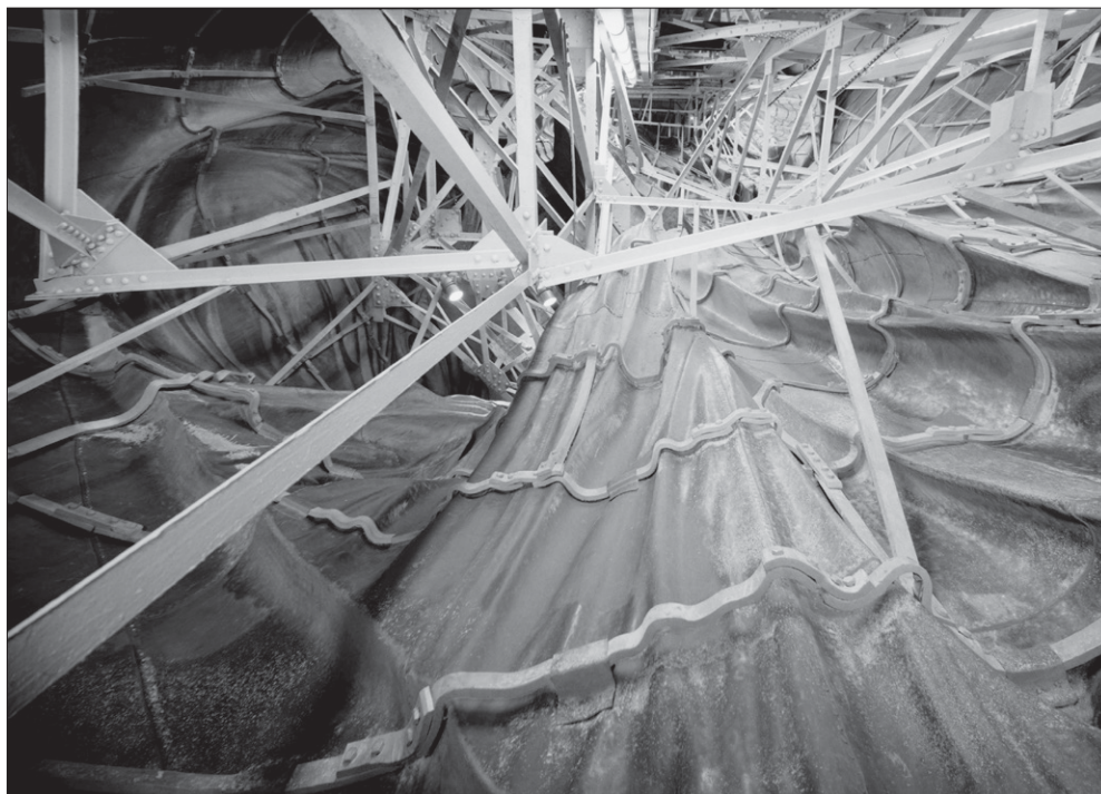
Figure 7 • Interior armature of the Statue of Liberty, after renovation in the 1980s. Source: National Institute of Standards and Technology (NIST) / Library of Congress.
