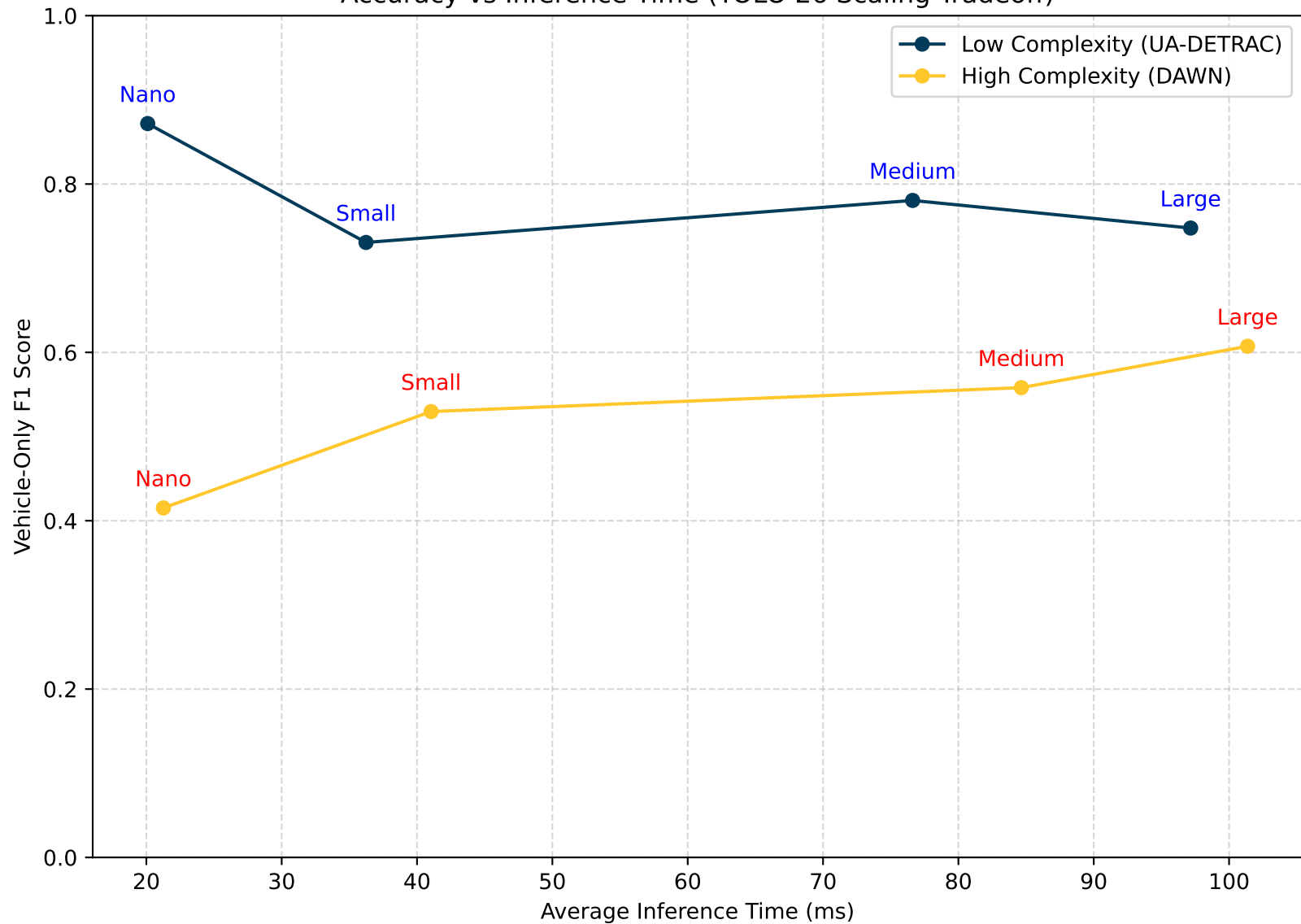
Accuracy vs Inference Time (YOLO 26 Scaling Tradeoff)
