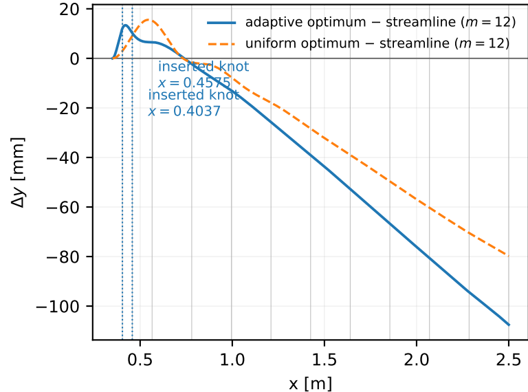
(b) what shape freedom bought at L = 2.5 m
