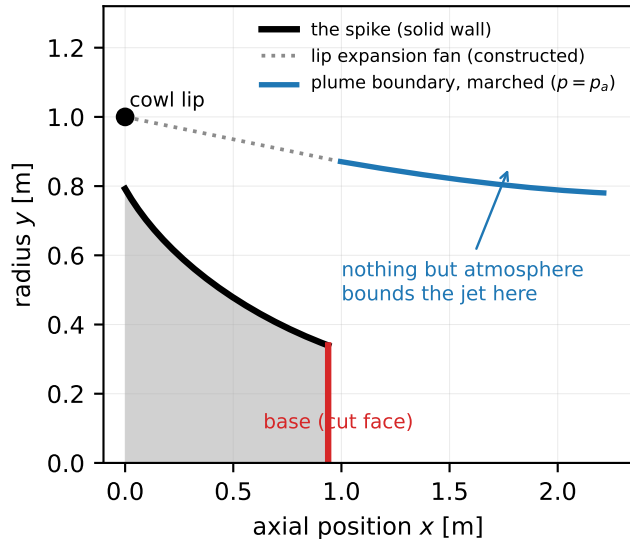
(b) the plug: the exhaust's outer edge is a free boundary, not a wall
