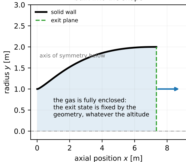
(a) the bell: one design point, built into the shape
