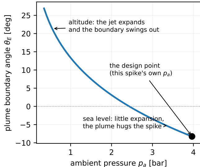
(c) altitude compensation, computed: the plume re-shapes itself with p_a
