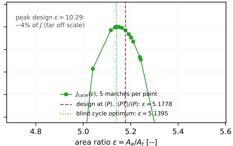
(b) mock RDE ( P and T profiles): one-number design within 2.5 \times 10^{-6}
