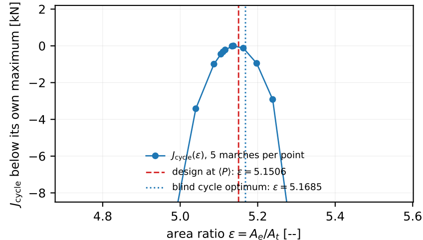
(a) pressure-only blowdown: zero gain over mean-pressure design (collapse)
