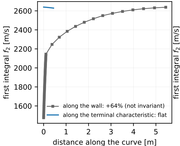
(b) f_2 is invariant ONLY on the characteristic
