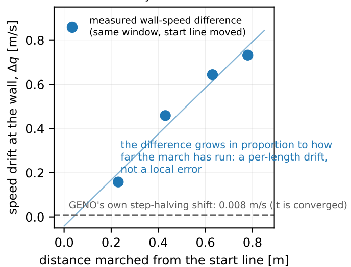
(c) the measured gap: linear in length, 0.5\% of the axisymmetric source effect
