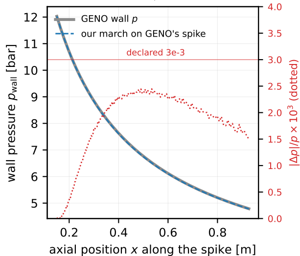
(a) the wall twin: two independent constructions, one contour
