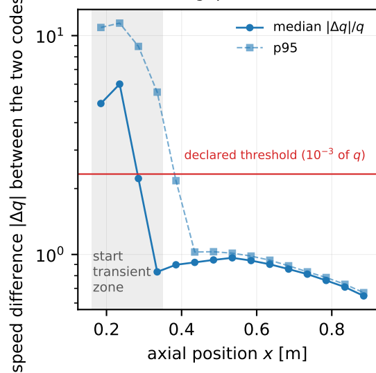
(b) the field twin: transient washes out, settled gap \approx 4 \times 10^{-4}
